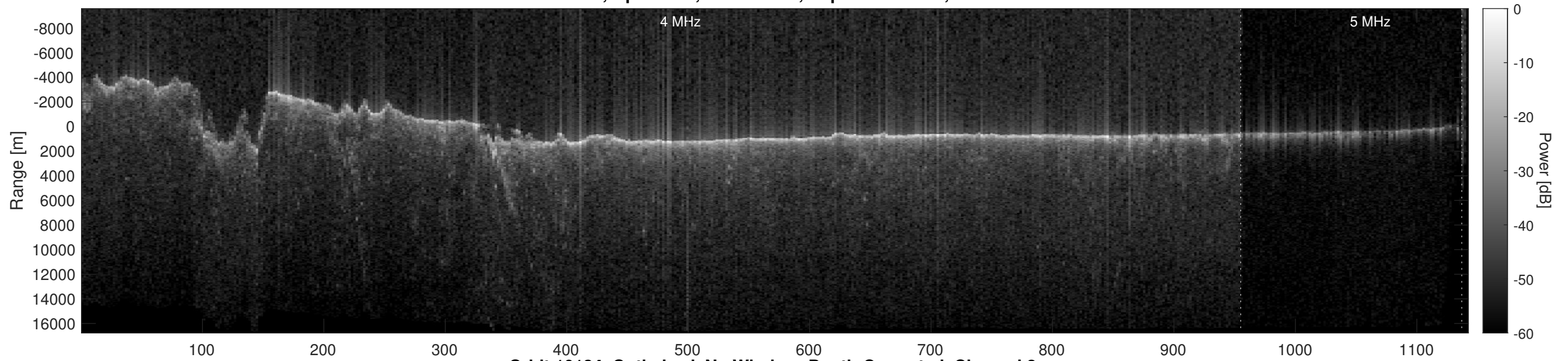
Orbit 10134, Optimized, No Window, Depth-Corrected, Channel 2
