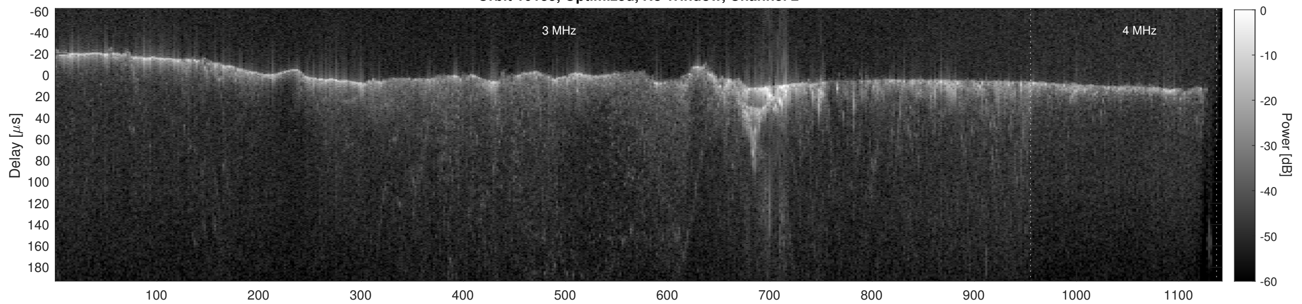
Orbit 10135, Cluttergram
