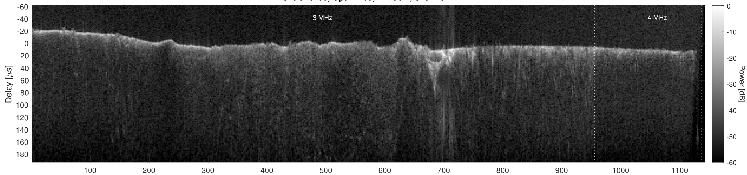
Orbit 10135, Cluttergram
