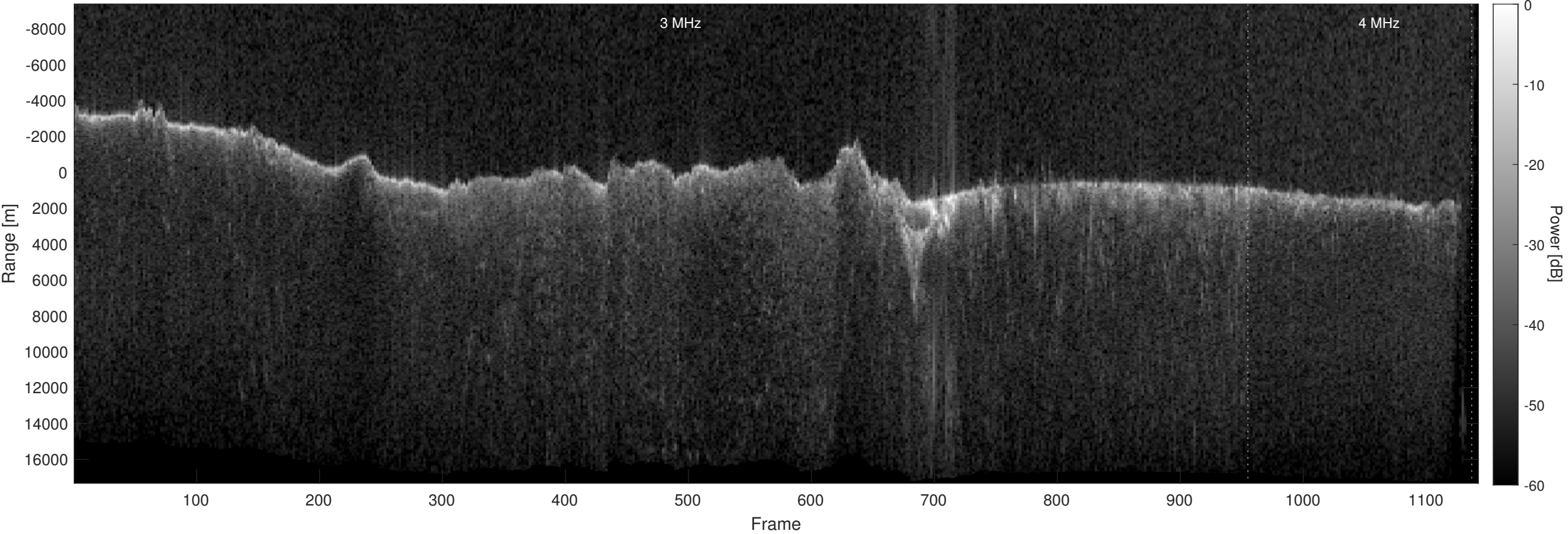
Orbit 10135, Optimized, Window, Depth-Corrected, Channel 2
