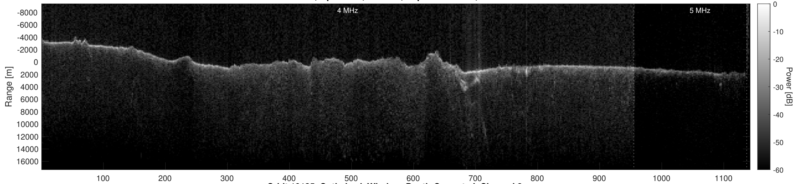
Orbit 10135, Optimized, Window, Depth-Corrected, Channel 2
