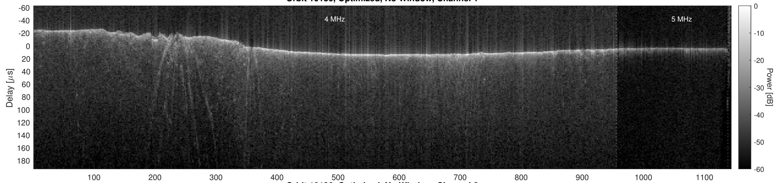
Orbit 10136, Optimized, No Window, Channel 2
