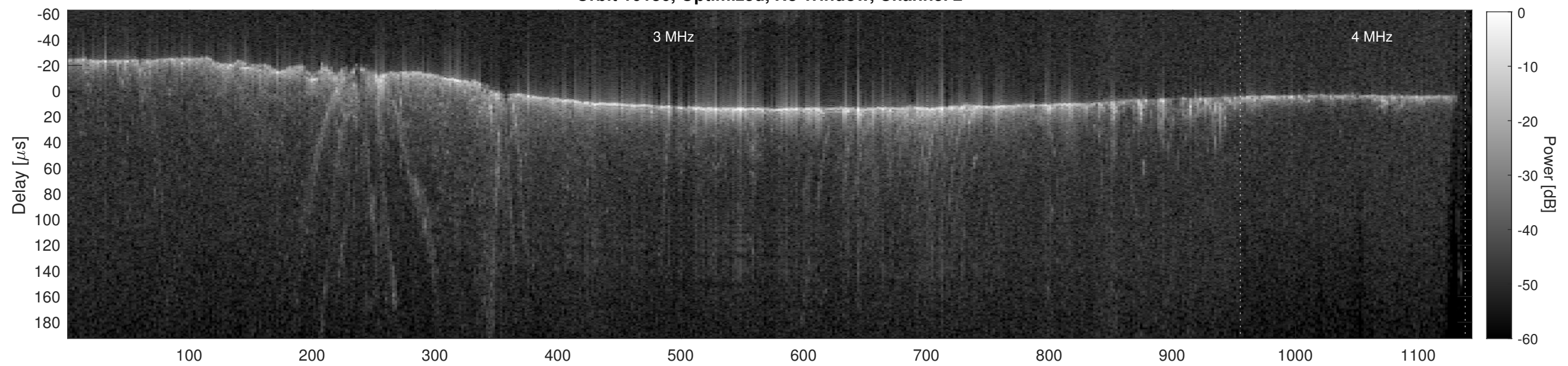
Orbit 10136, Cluttergram
