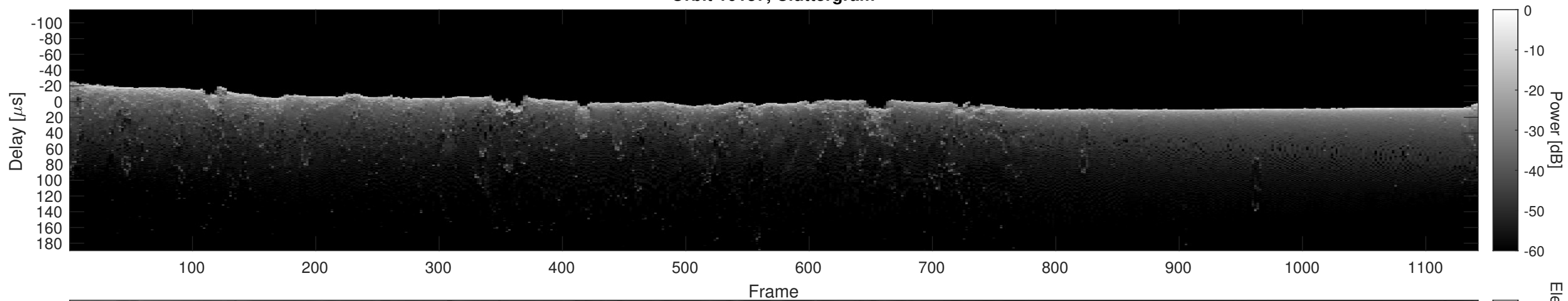
Orbit 10137, Cluttergram
