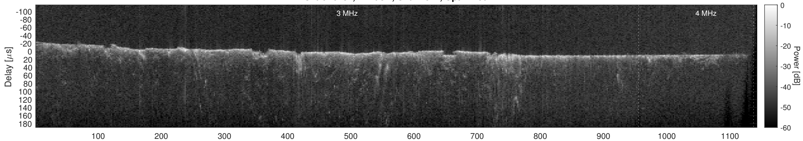
Orbit 10137, Cluttergram
