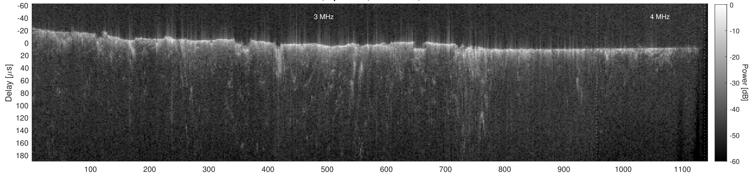
Orbit 10137, Cluttergram
