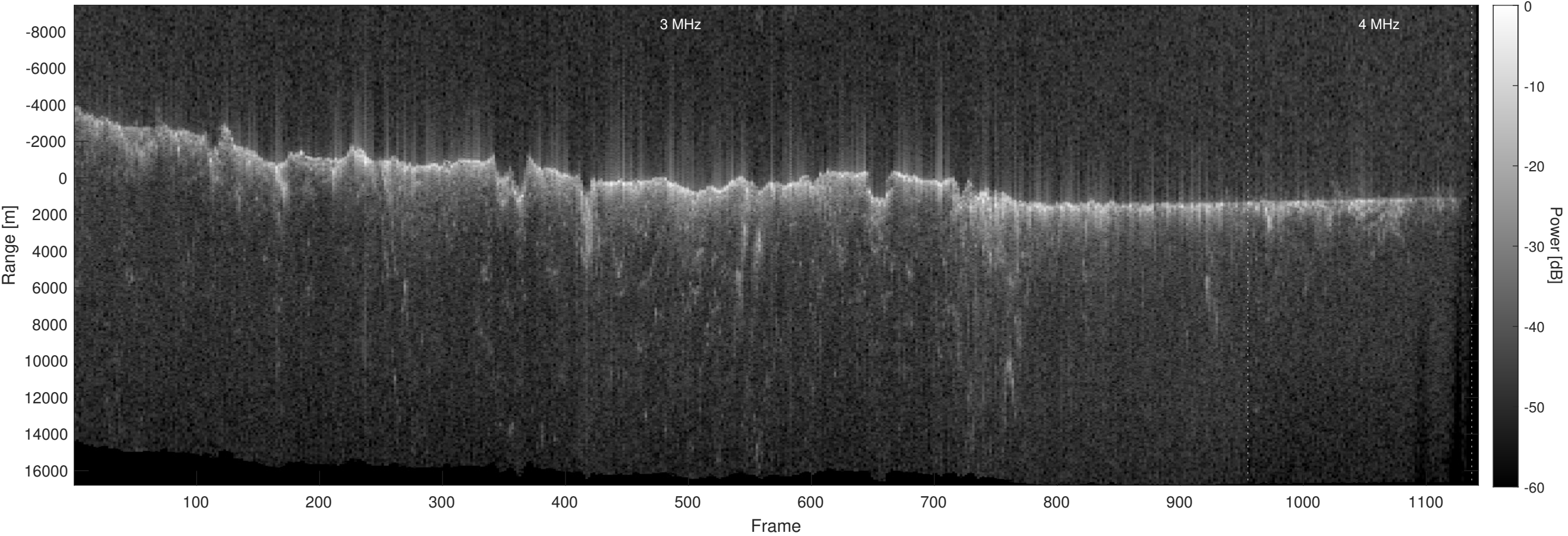
Orbit 10137, Optimized, No Window, Depth-Corrected, Channel 2
