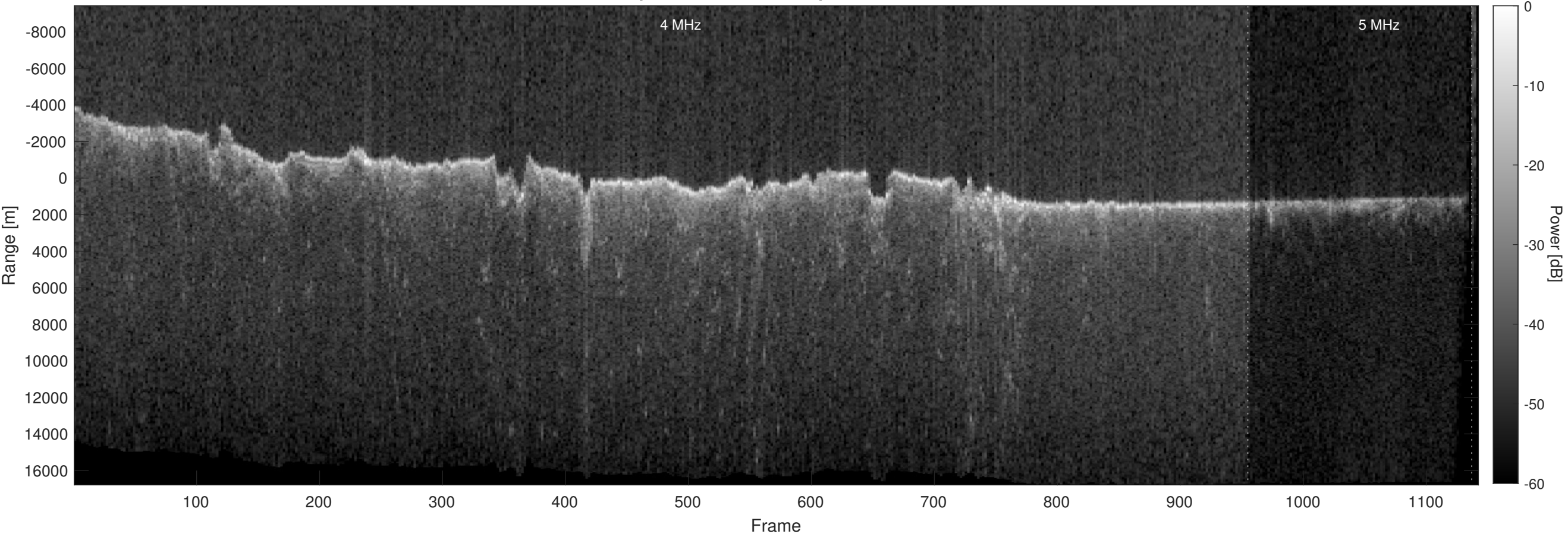
Orbit 10137, Optimized, Window, Depth-Corrected, Channel 2
