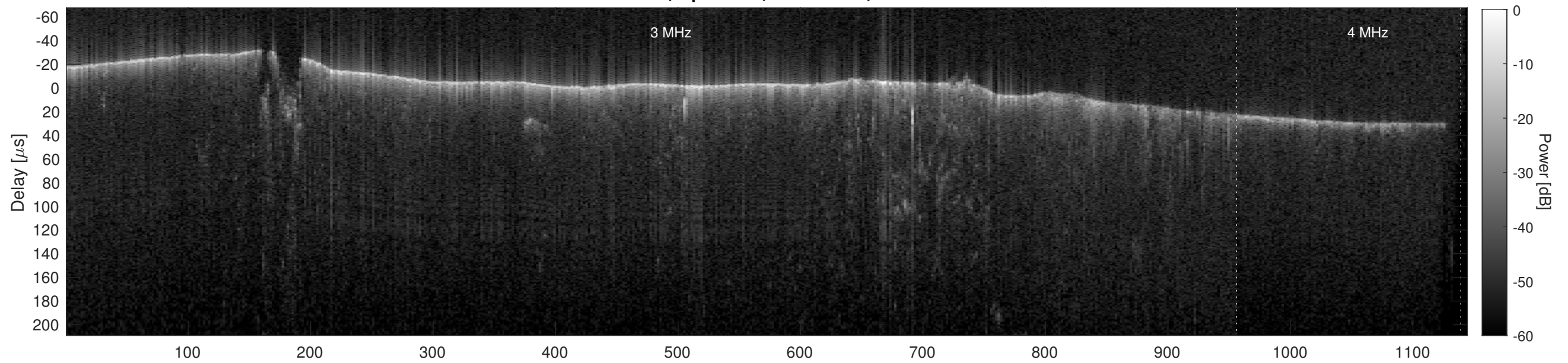
Orbit 10138, Cluttergram
