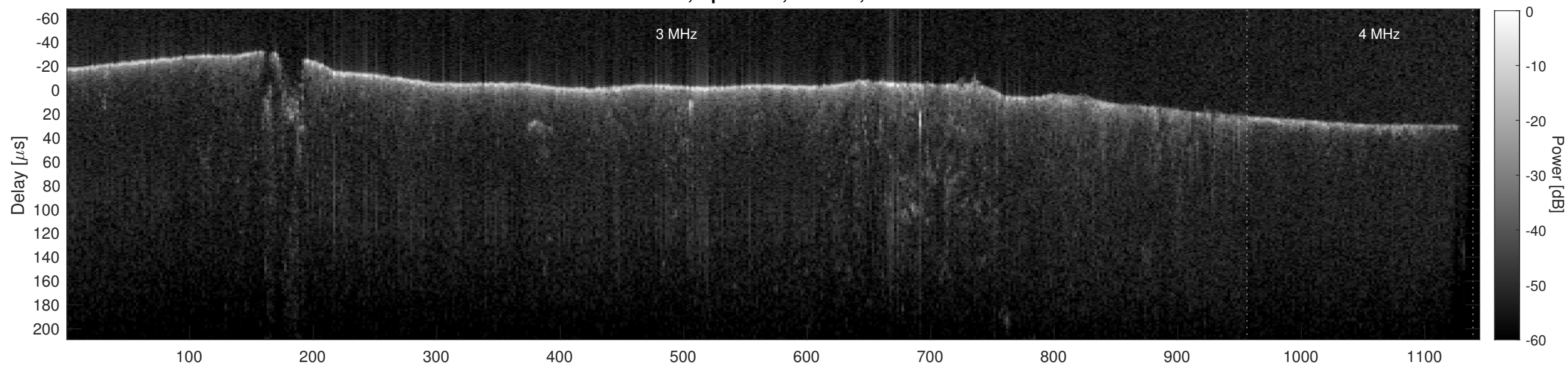
Orbit 10138, Cluttergram
