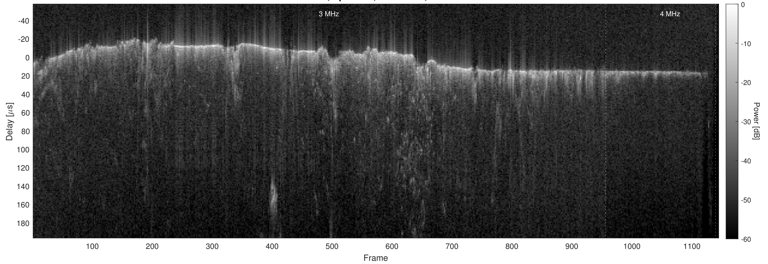
Orbit 10140, Optimized, No Window, Channel 2
