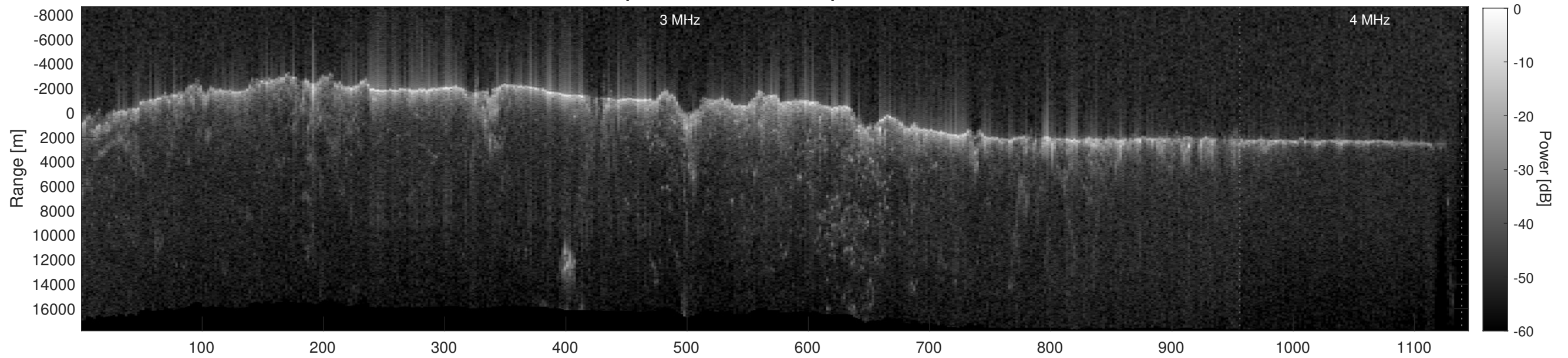
Orbit 10140, Depth-Corrected Cluttergram
