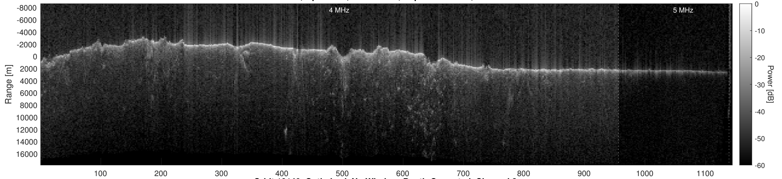
Orbit 10140, Optimized, No Window, Depth-Corrected, Channel 2
