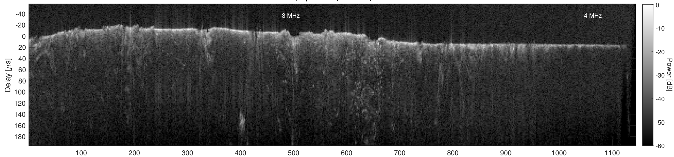
Orbit 10140, Cluttergram
