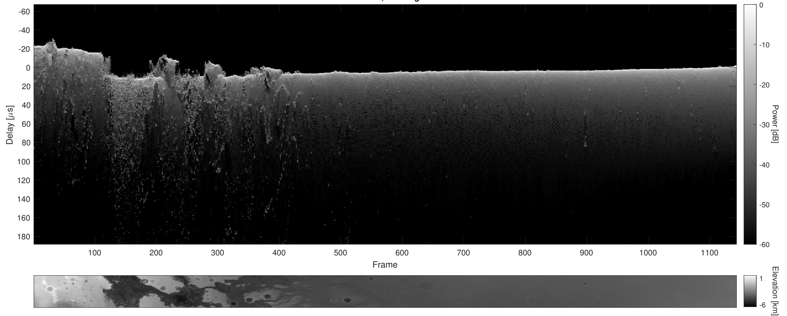
Orbit 10141, Cluttergram
