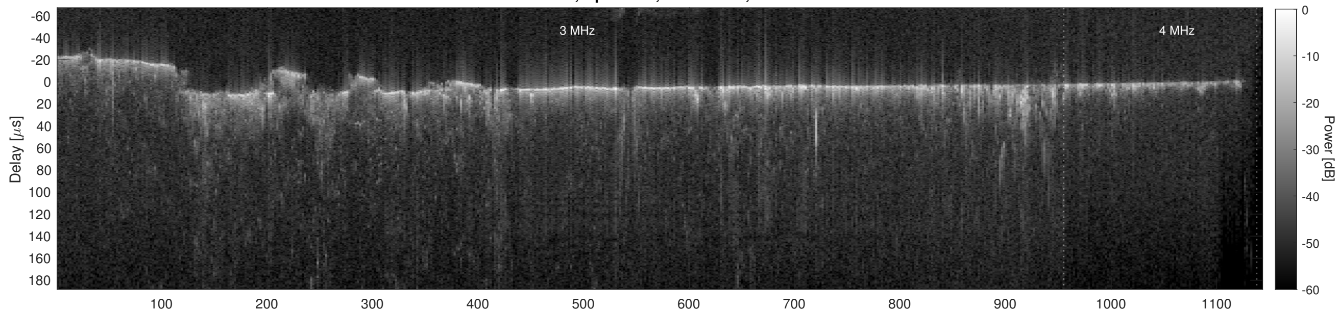
Orbit 10141, Cluttergram
