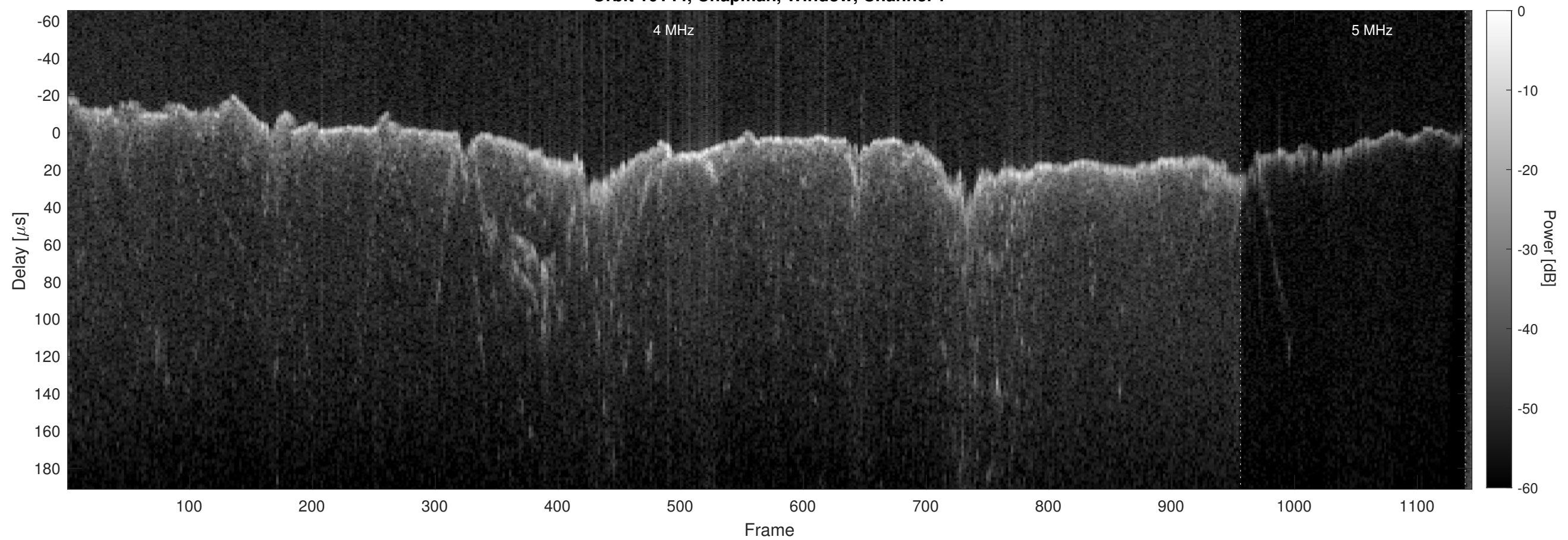
Orbit 10144, Chapman, Window, Channel 2
