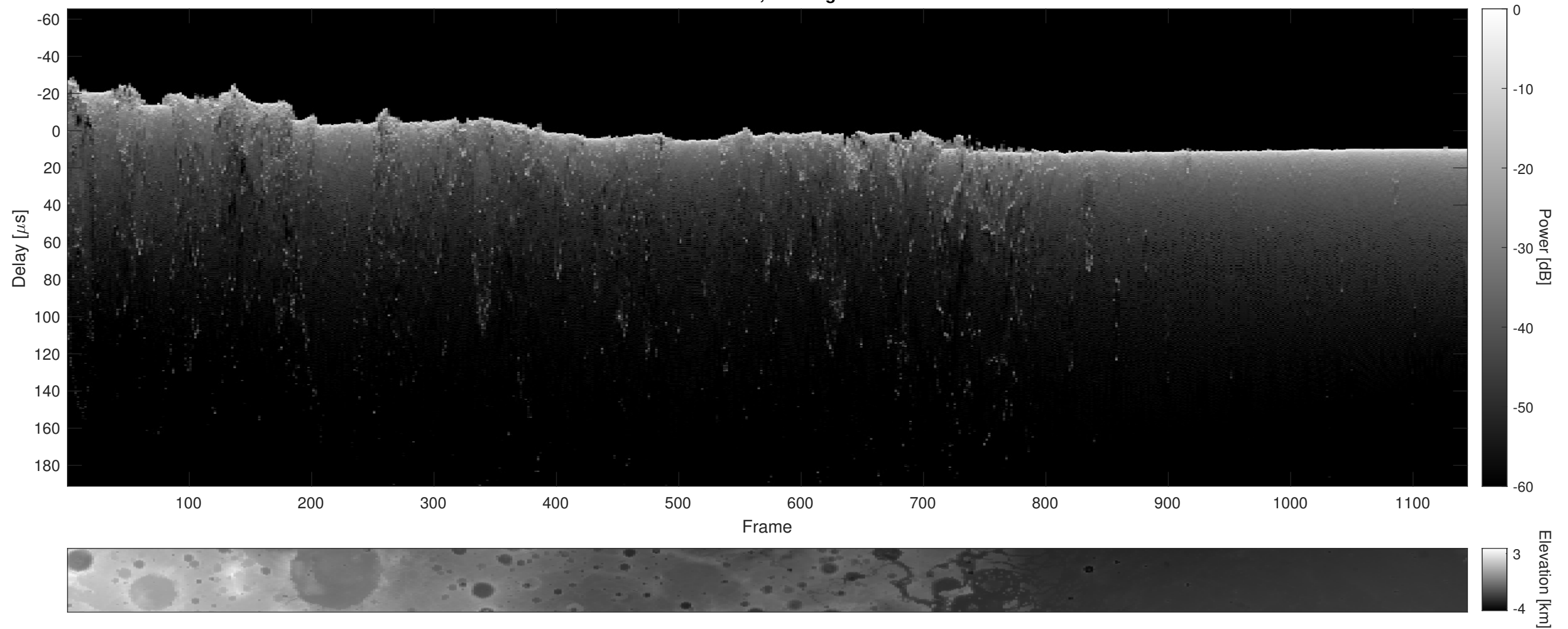
Orbit 10144, Cluttergram
