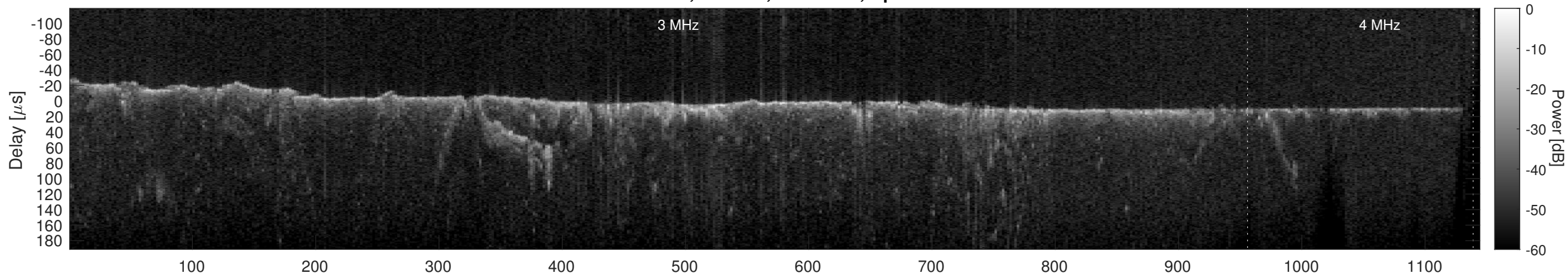
Orbit 10144, Cluttergram
