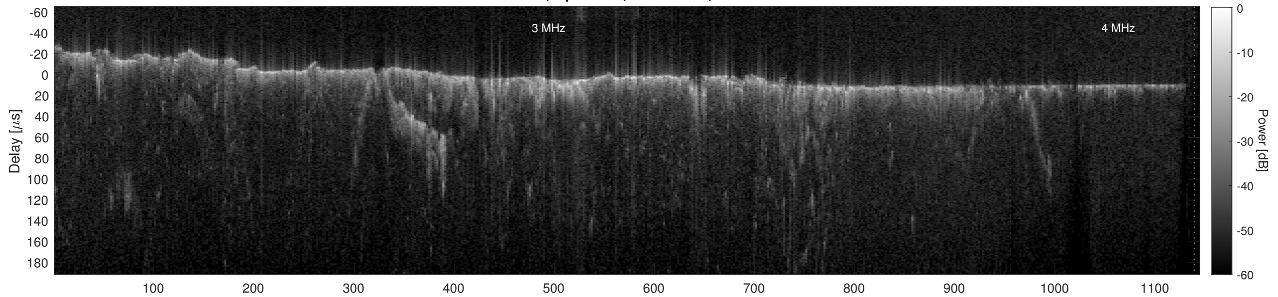
Orbit 10144, Cluttergram
