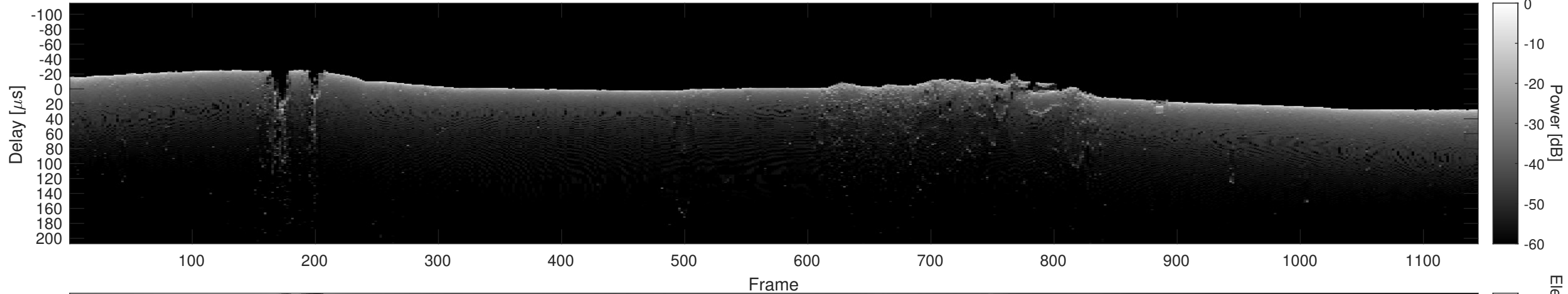
Orbit 10145, Cluttergram
