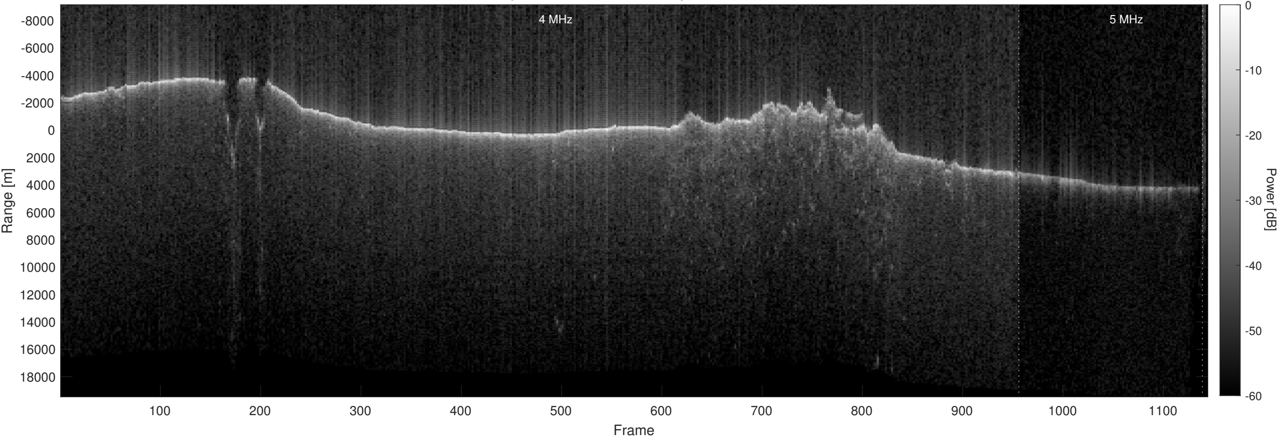
Orbit 10145, Optimized, No Window, Depth-Corrected, Channel 2
