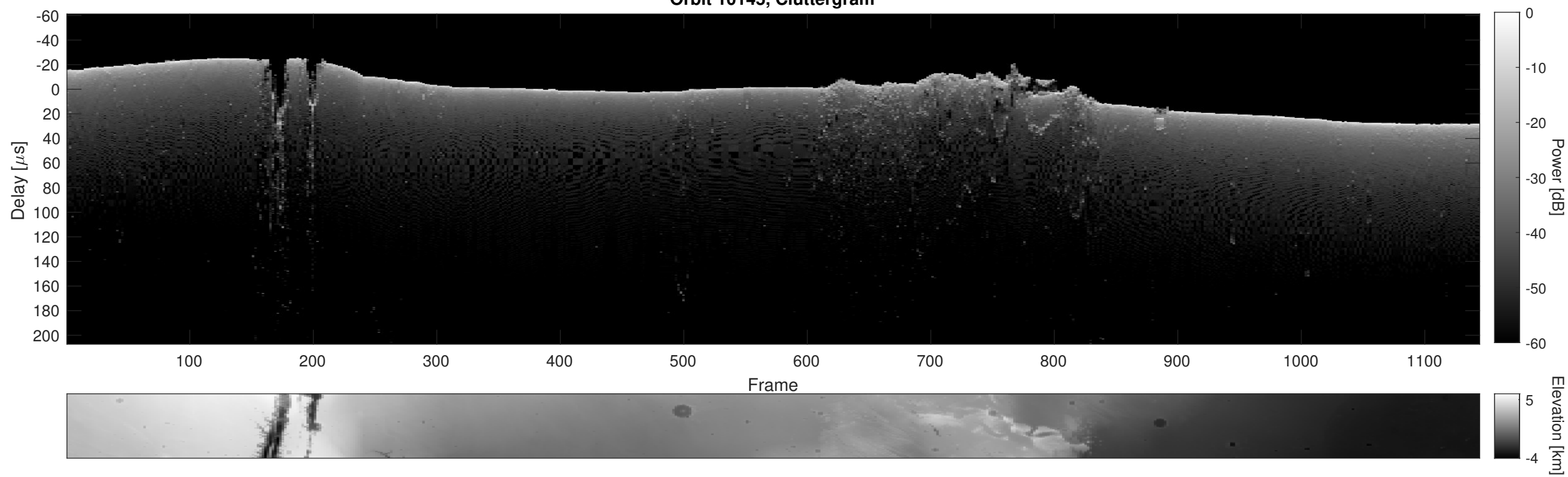
Orbit 10145, Cluttergram
