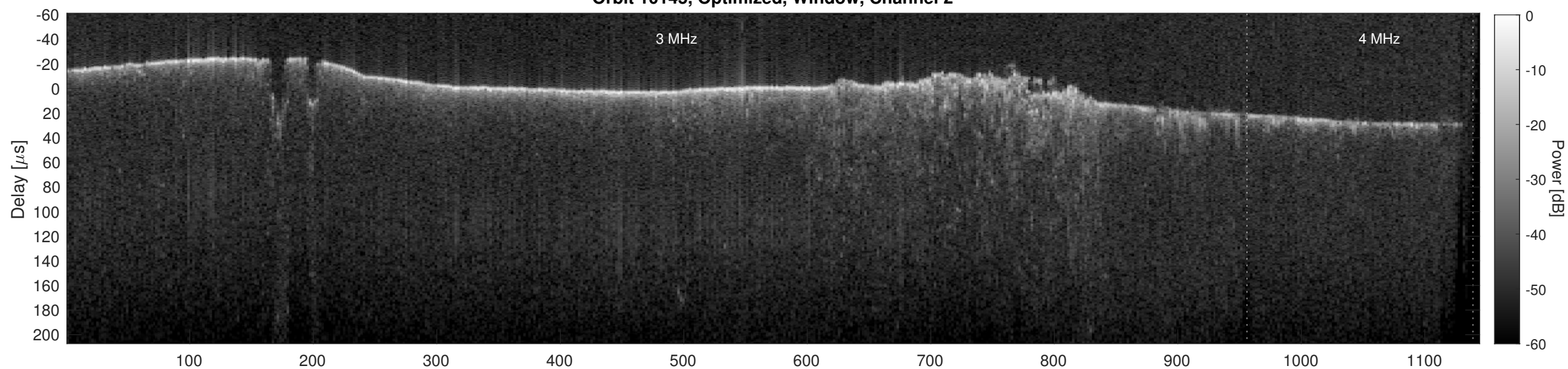
Orbit 10145, Cluttergram
