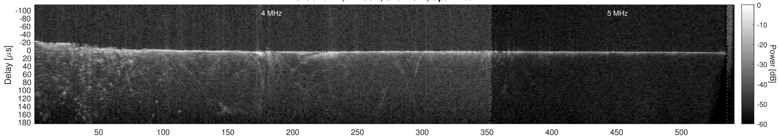
Orbit 10147, Cluttergram
