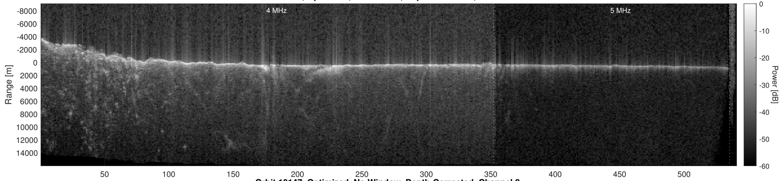
Orbit 10147, Optimized, No Window, Depth-Corrected, Channel 2
