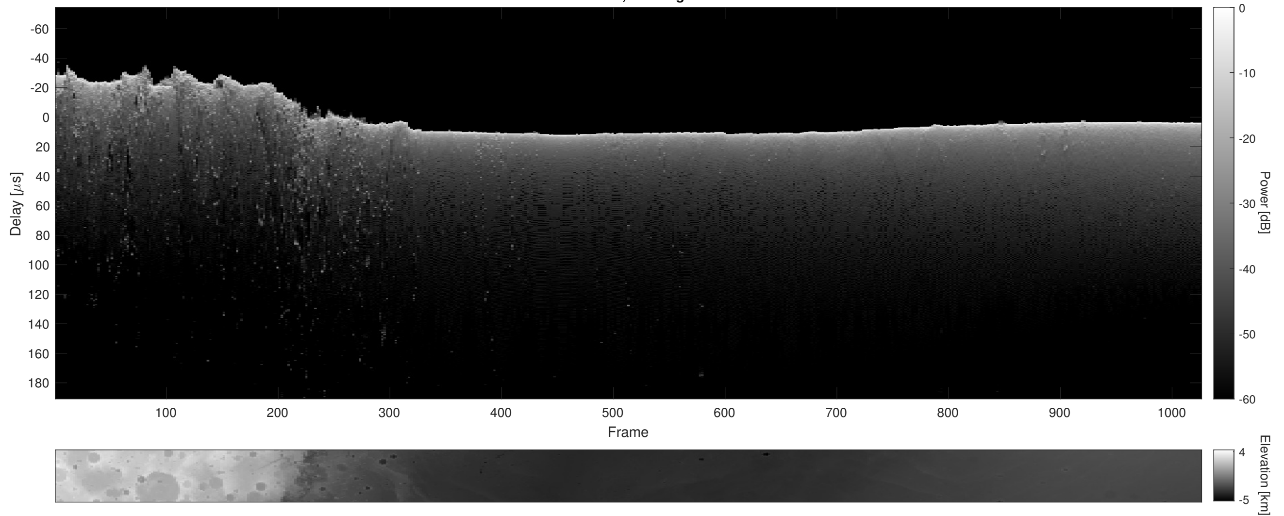
Orbit 10157, Cluttergram
