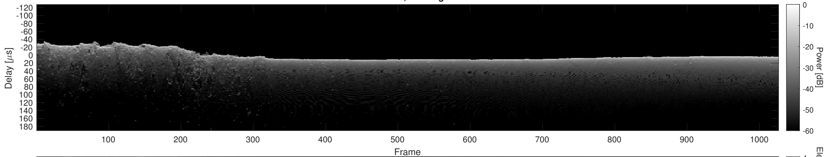
Orbit 10157, Cluttergram
