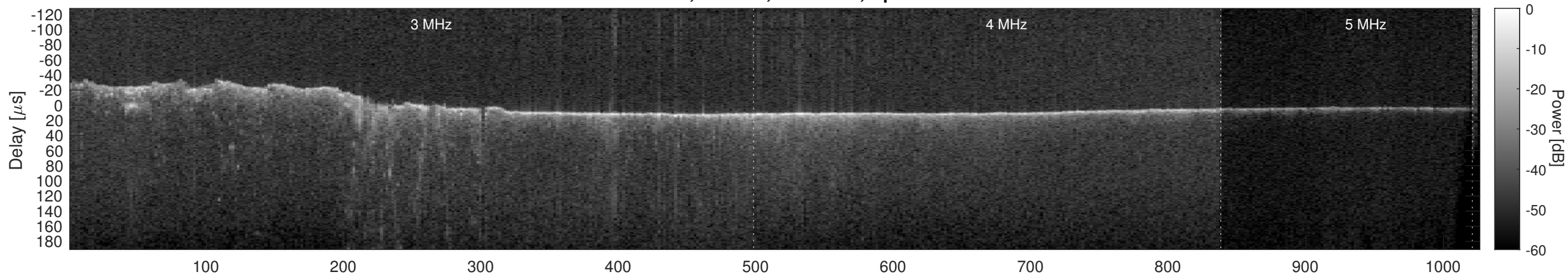
Orbit 10157, Cluttergram
