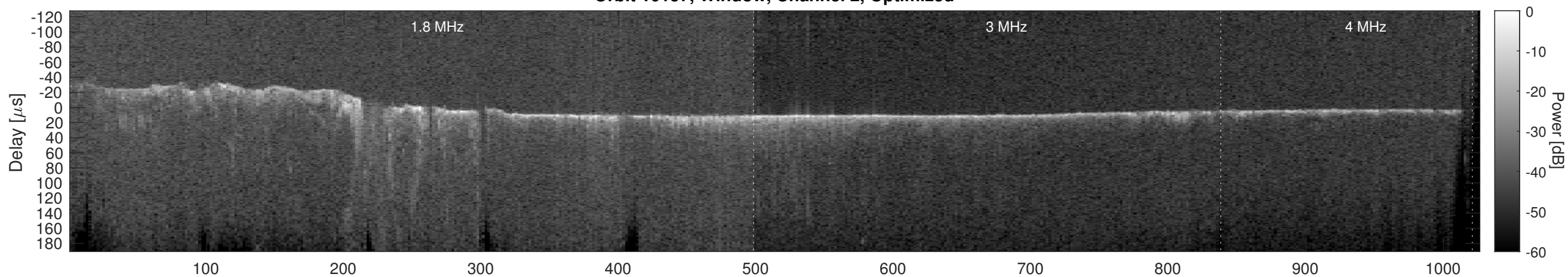
Orbit 10157, Cluttergram
