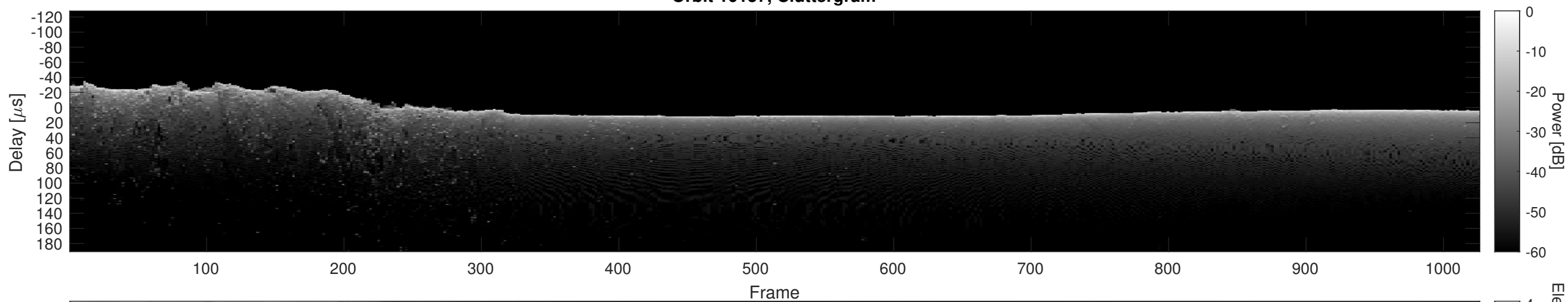
Orbit 10157, Cluttergram
