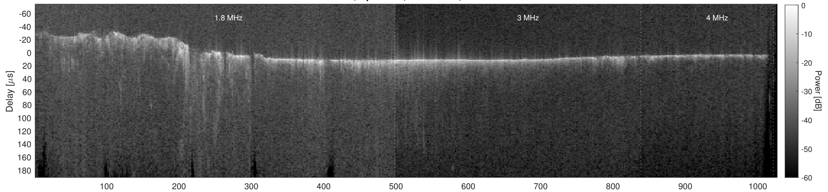
Orbit 10157, Cluttergram
