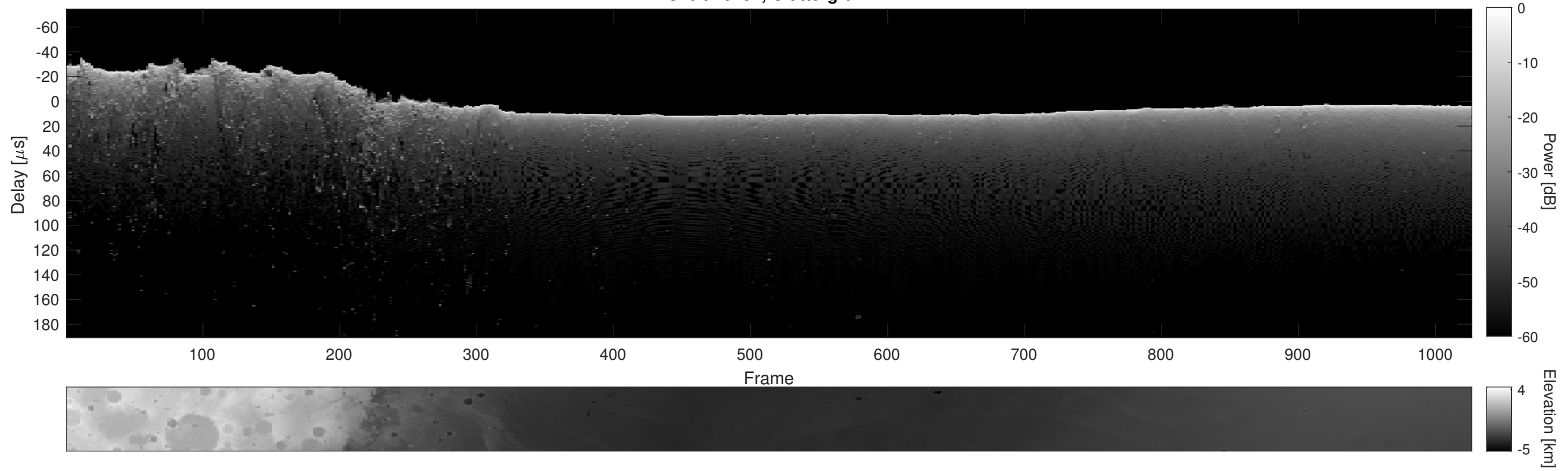
Orbit 10157, Cluttergram
