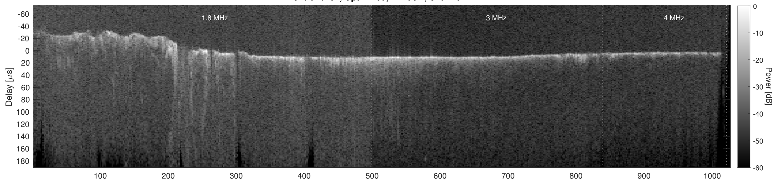
Orbit 10157, Cluttergram
