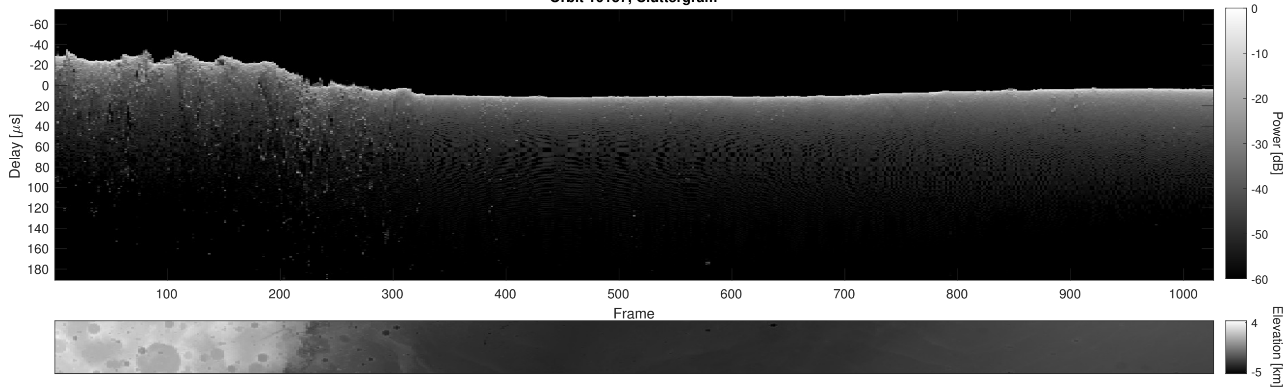
Orbit 10157, Cluttergram
