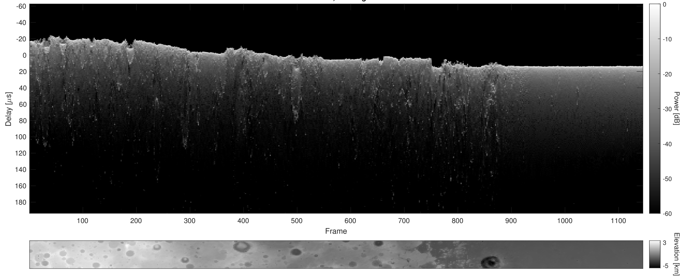
Orbit 10158, Cluttergram
