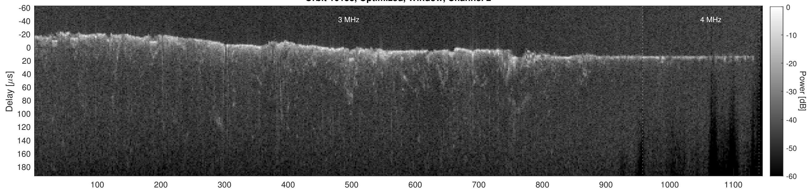
Orbit 10158, Cluttergram
