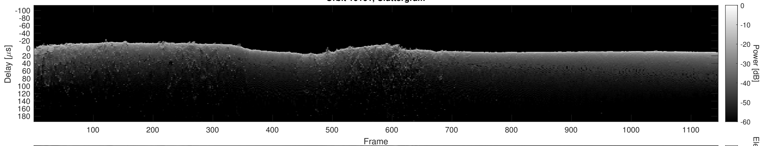
Orbit 10161, Cluttergram
