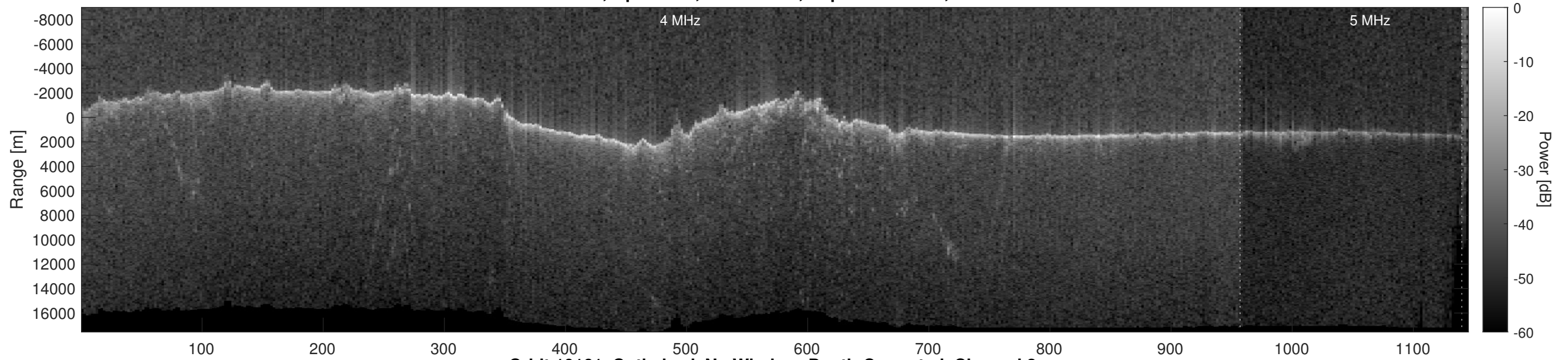
Orbit 10161, Optimized, No Window, Depth-Corrected, Channel 2
