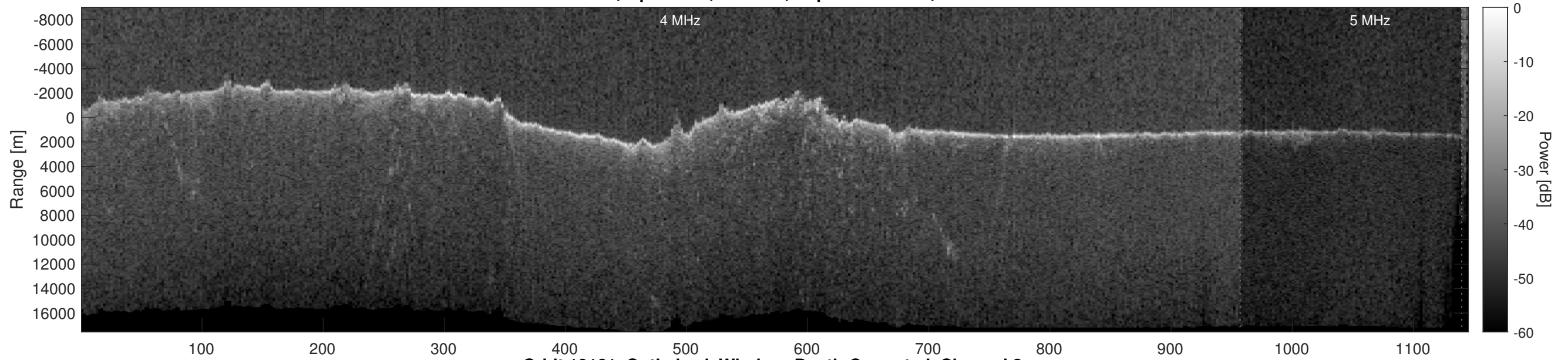
Orbit 10161, Optimized, Window, Depth-Corrected, Channel 2
