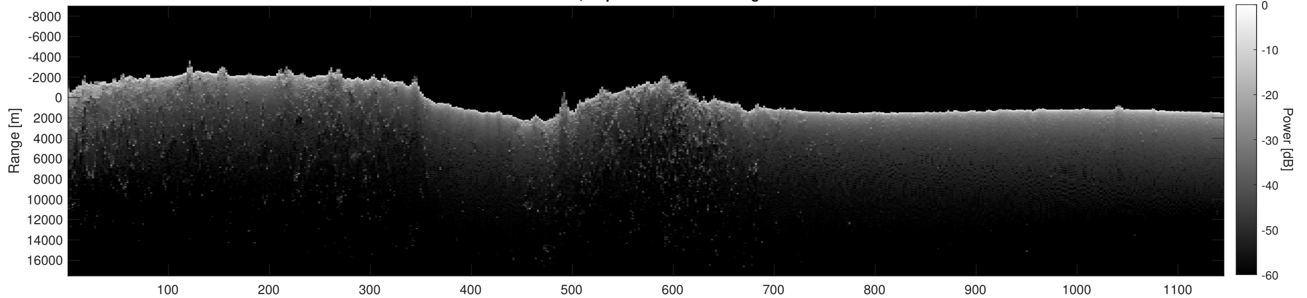
Orbit 10161, Depth-Corrected Cluttergram
