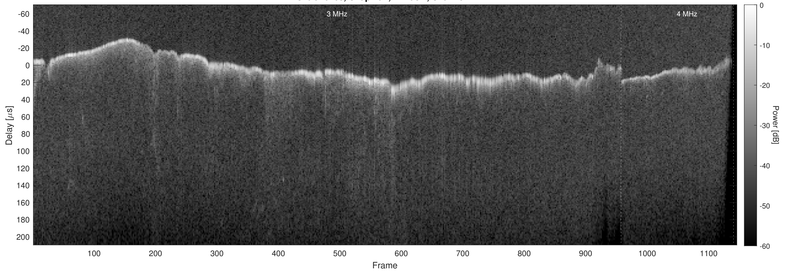
Orbit 10163, Chapman, Window, Channel 2
