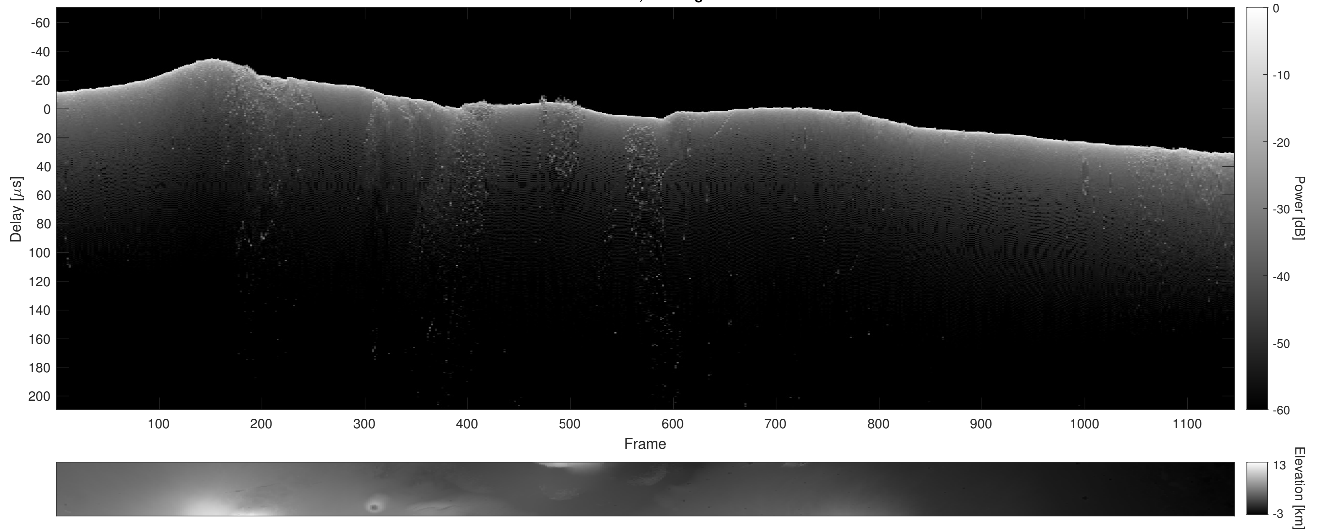
Orbit 10163, Cluttergram
