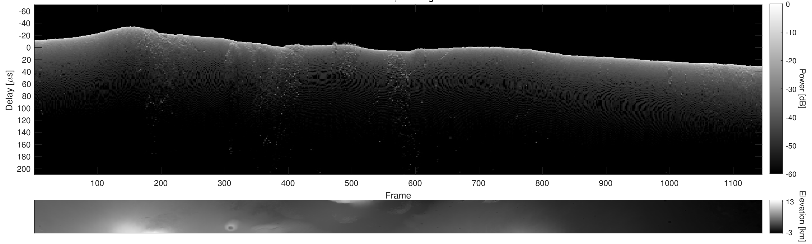
Orbit 10163, Cluttergram
