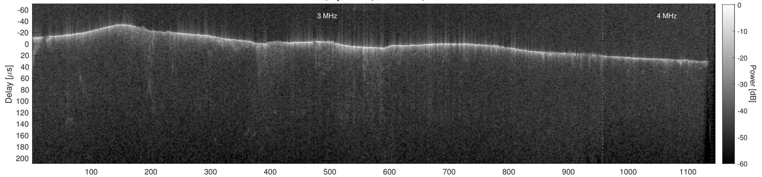
Orbit 10163, Cluttergram
