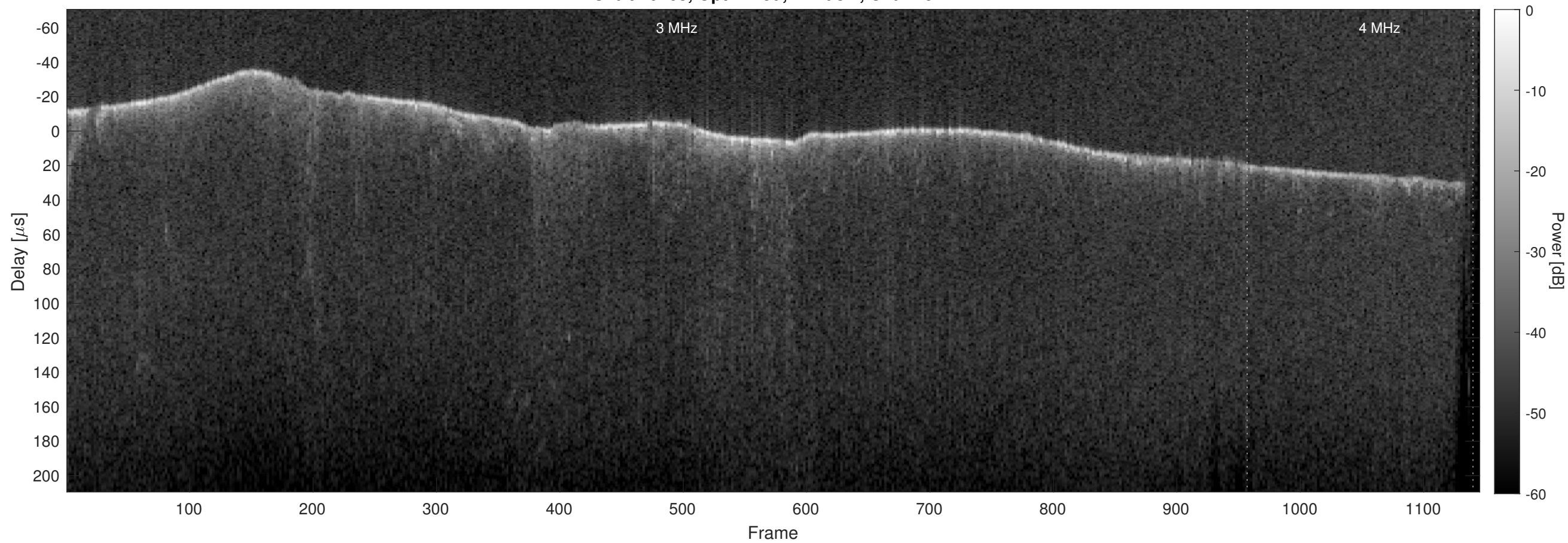
Orbit 10163, Optimized, Window, Channel 2
