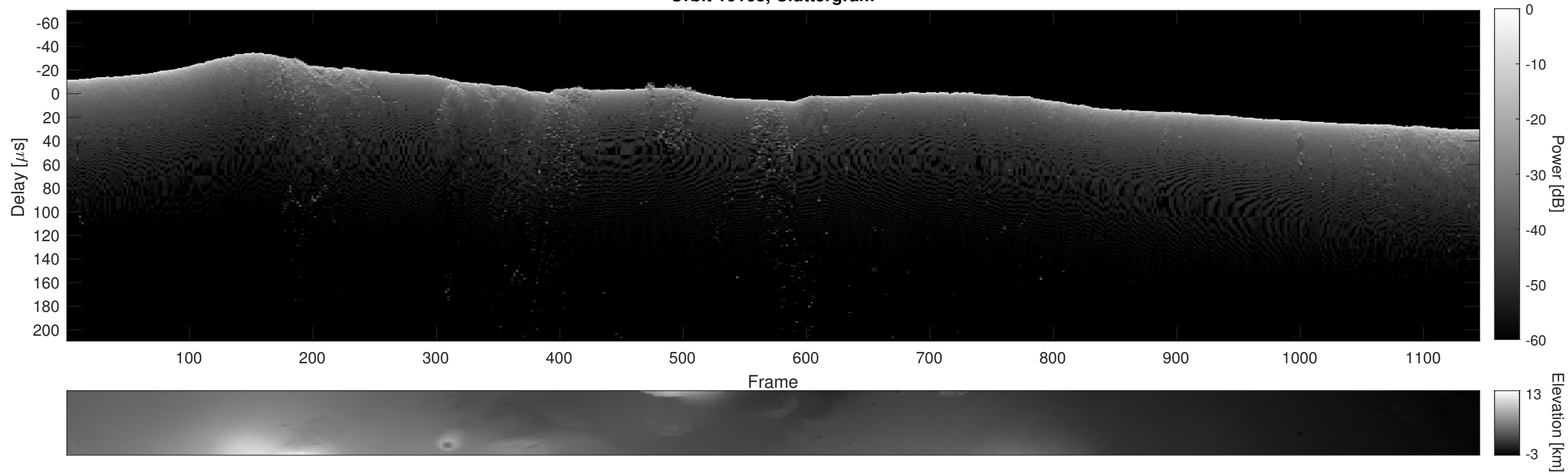
Orbit 10163, Cluttergram
