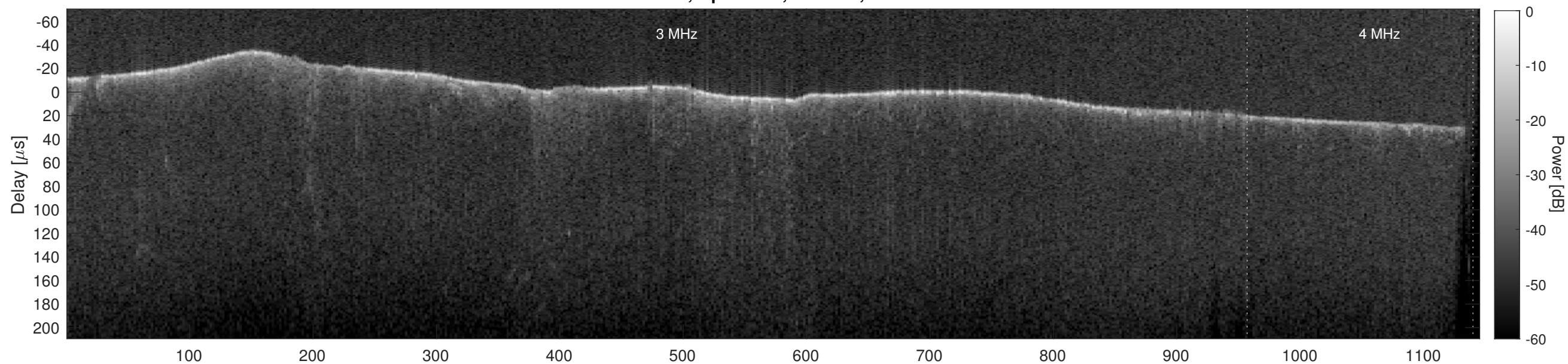
Orbit 10163, Cluttergram
