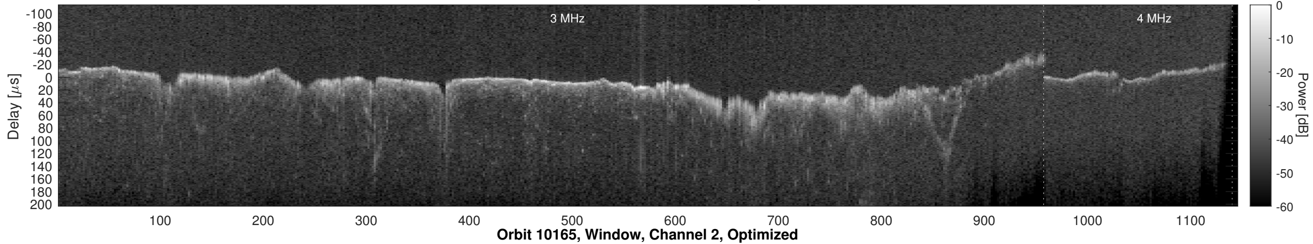
Orbit 10165, Window, Channel 2, Chapman
