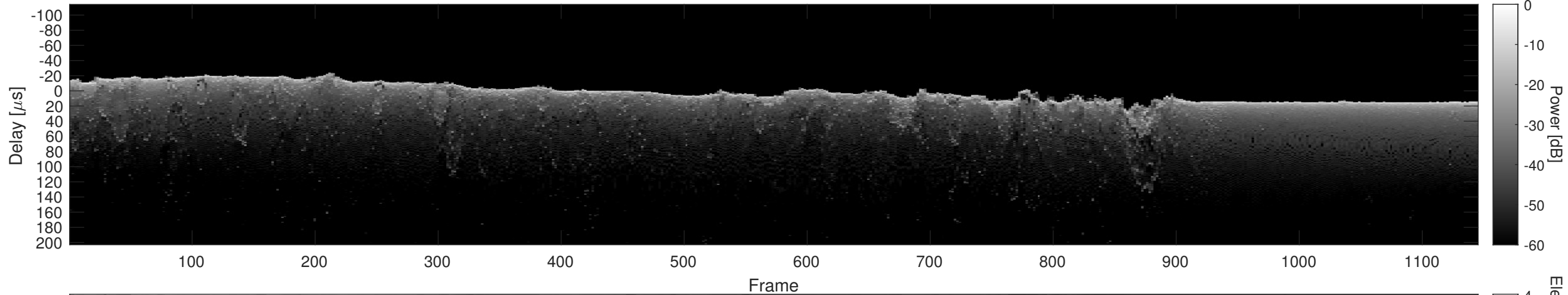
Orbit 10165, Cluttergram
