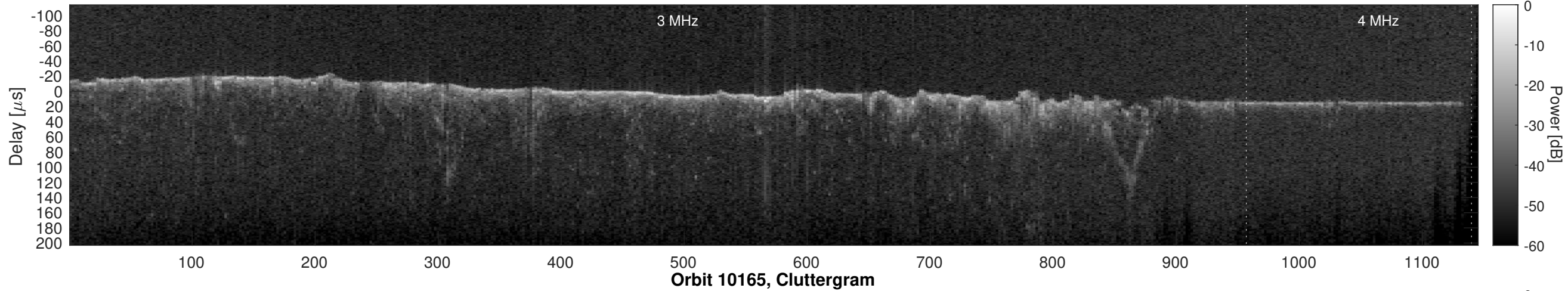
Orbit 10165, Window, Channel 2, Optimized
