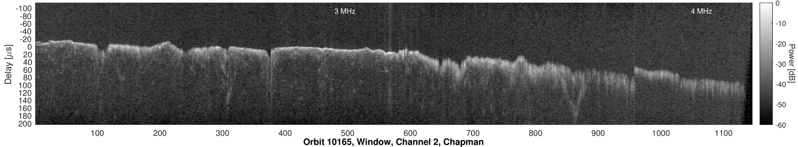
Orbit 10165, Window, Channel 2, Uncorrected
