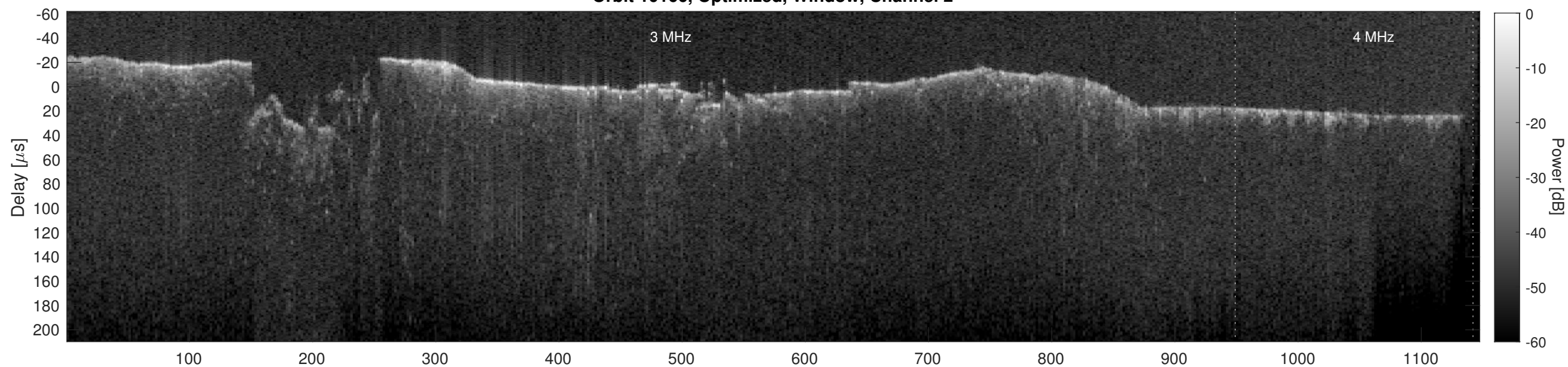
Orbit 10166, Cluttergram
