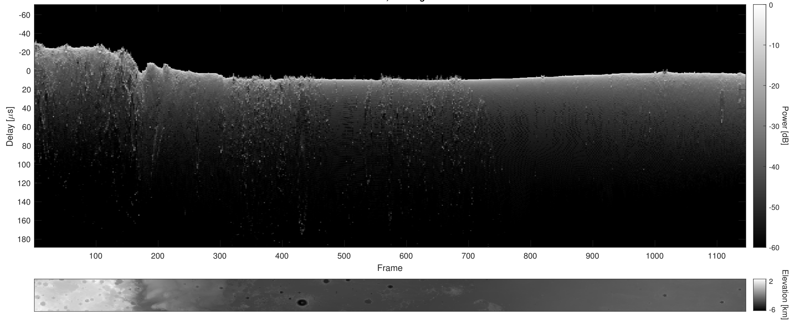
Orbit 10167, Cluttergram
