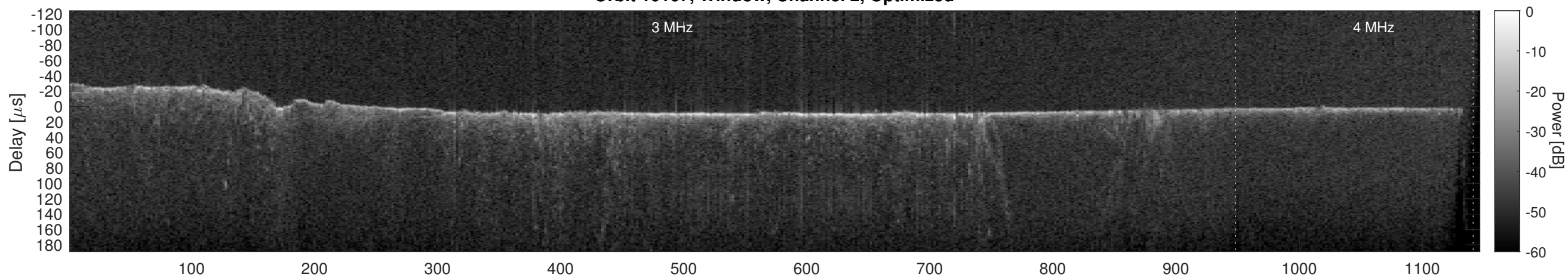
Orbit 10167, Cluttergram
