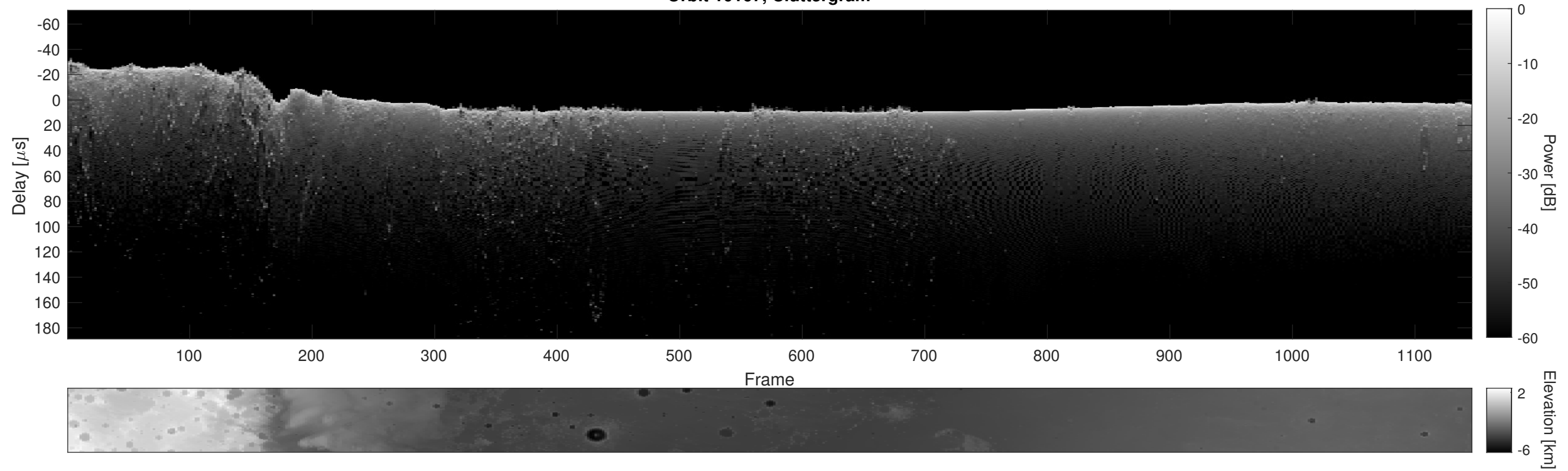
Orbit 10167, Cluttergram
