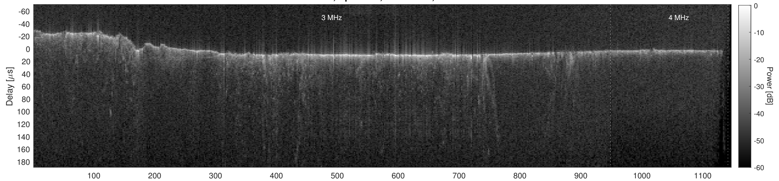
Orbit 10167, Cluttergram
