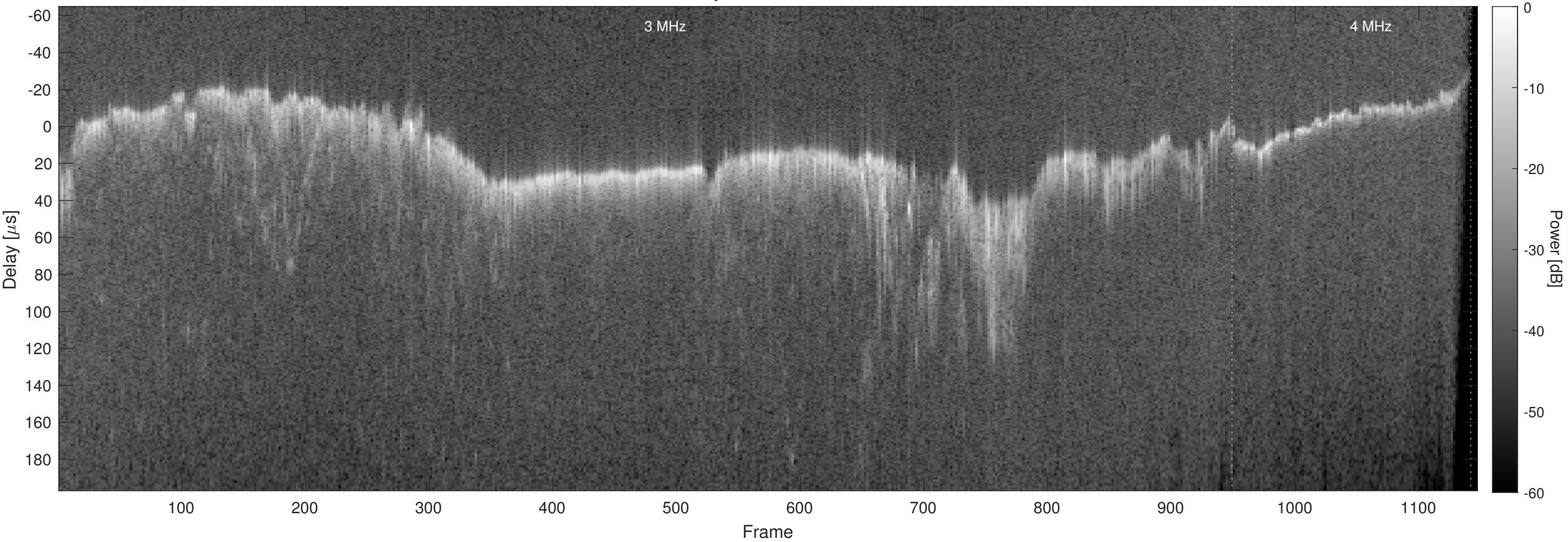
Orbit 10168, Chapman, No Window, Channel 2
