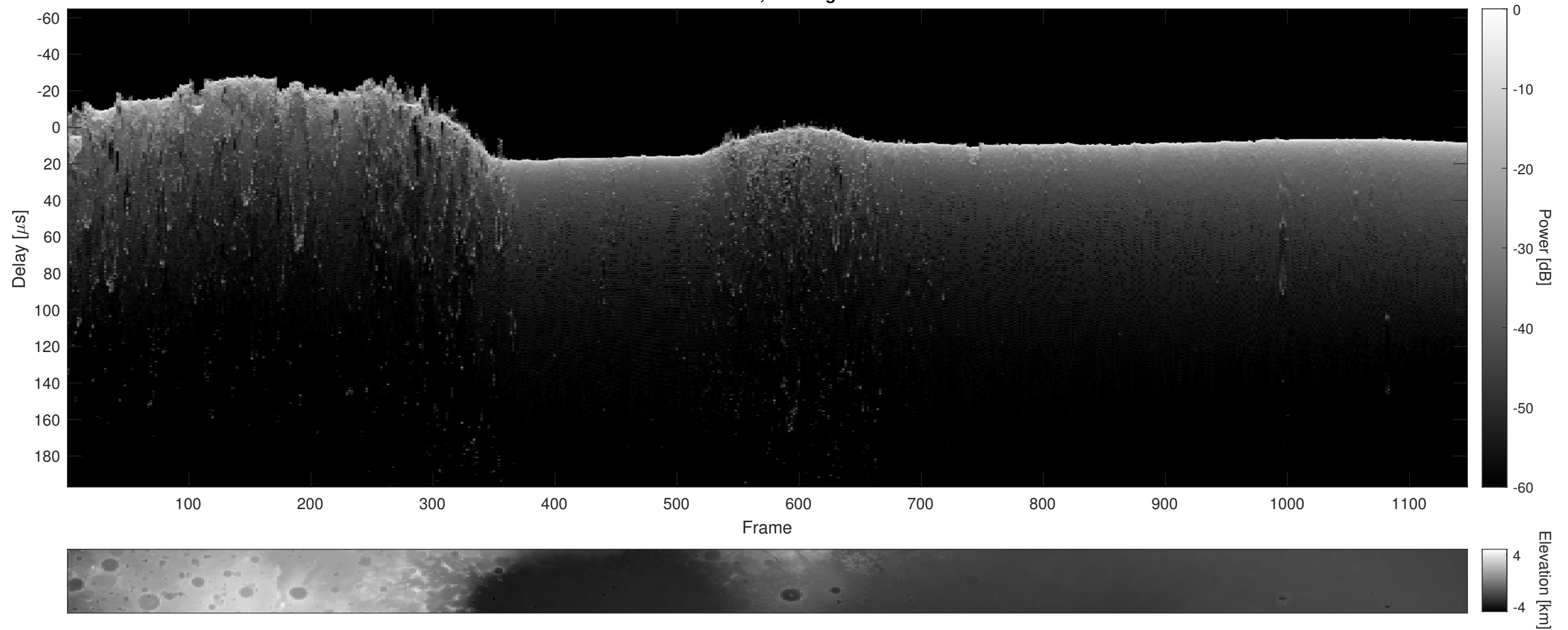
Orbit 10168, Cluttergram
