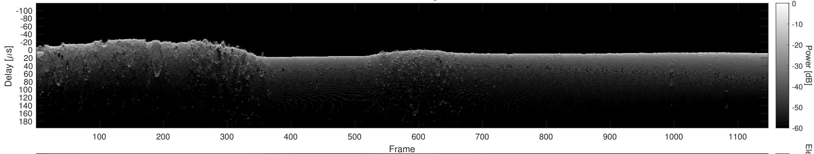
Orbit 10168, Cluttergram
