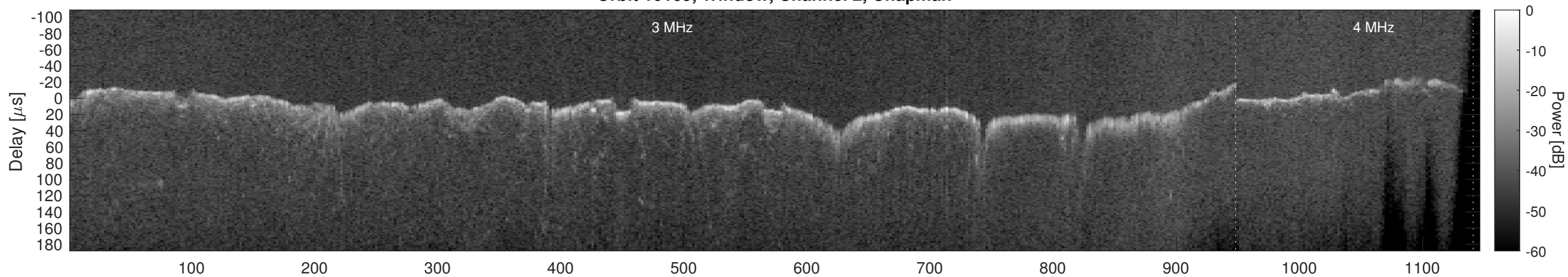
Orbit 10169, Window, Channel 2, Optimized
