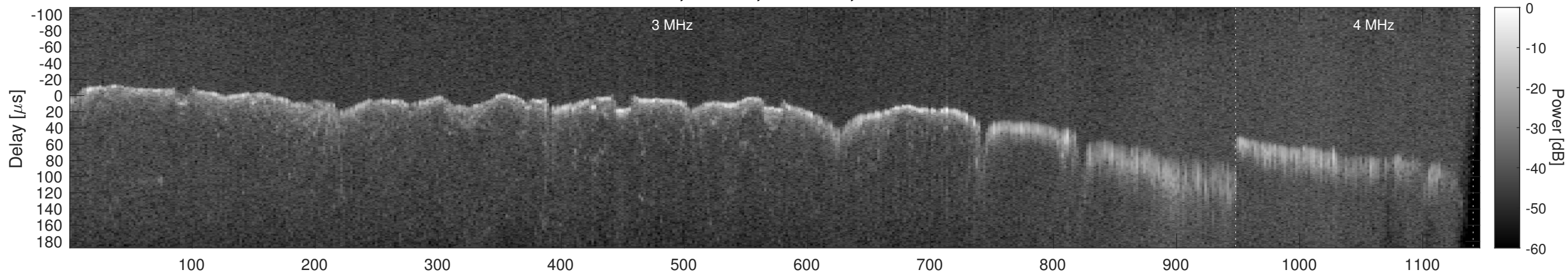
Orbit 10169, Window, Channel 2, Chapman
